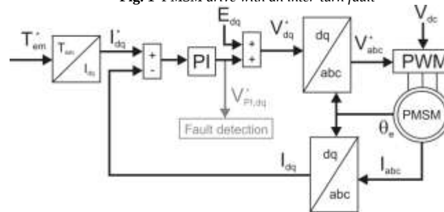
Fig. 1 PMSM drive with an inter-turn fault
