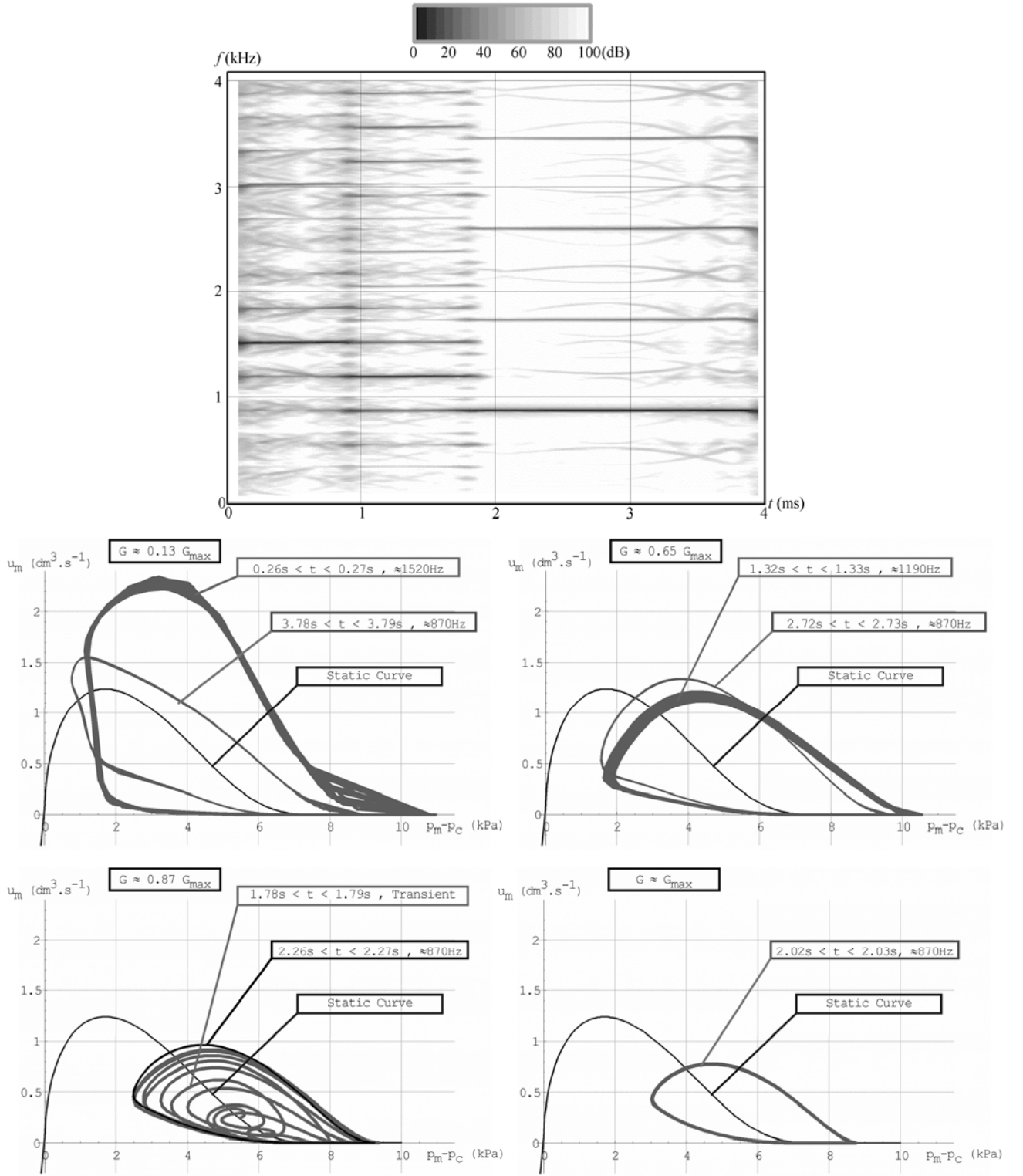
Figure 6: Time frequency analysis (spectrogram) and phase diagrams (p_m - p_c) \Leftrightarrow \text{flow } u_c of the sound recorded on Track 2 for the three modes of oscillation (partials 9, 7 and 5) and the transient between 2 nd and 3 rd modes. On each figure, adjustments are rigorously identical; only their past differs.
