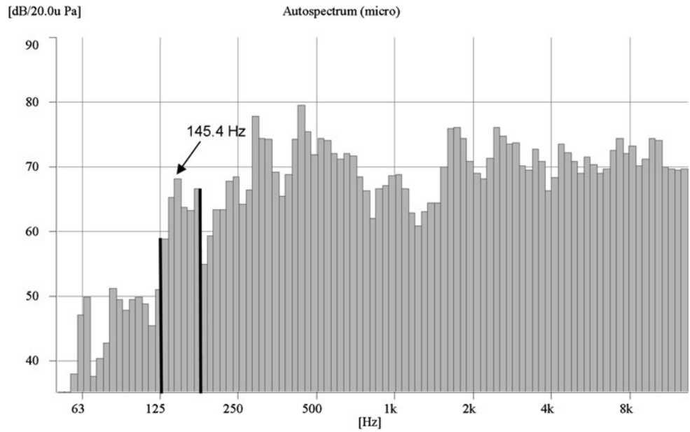
Fig. 6 1/12-octave band power spectrum from microphone signals for strongly checked poplar veneer
