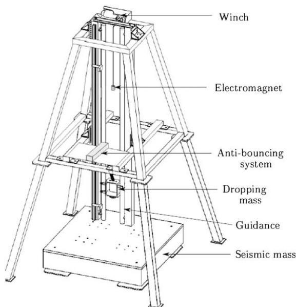
Fig. 2. Global drop tower.
