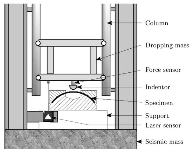
Fig. 3. Detailed drop tower.
