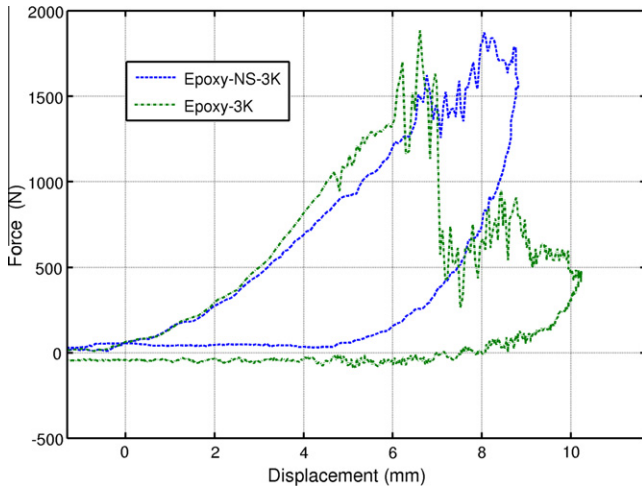
Fig. 7. Representative force vs. displacement behavior during impact on Epoxy-NS-3K and Epoxy-3K.
