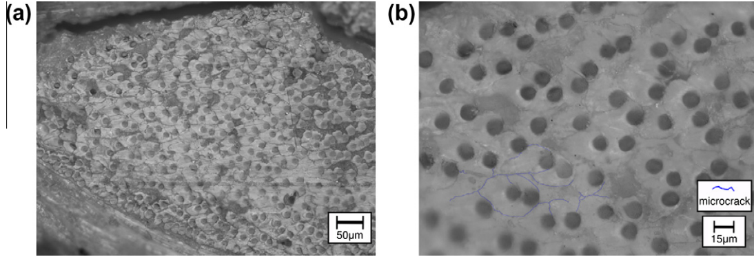
Fig. 13. Micrographs showing the significant rate of micro crack in the yarn located in the last ply of the composite structure.
