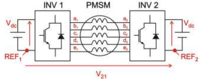
Fig. 1: Drive topology
