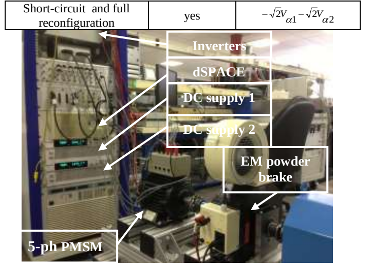
Fig. 6: Experimental platform.
