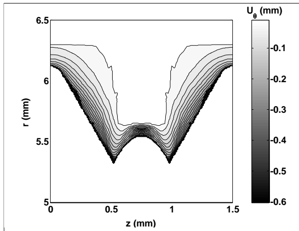
Figure 9. Tangential displacement U_{\theta}(r,z)
