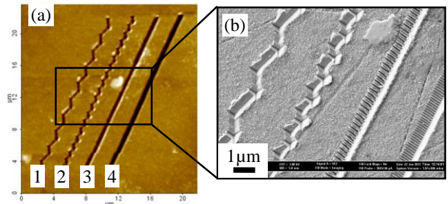
Fig. 6: Grooves machined using the Bresenham algorithm with different discretization steps: (a): AFM image, (b): SEM image. The discretization steps indicated on (a) are: groove (1): 1 \mu\text{m} ; (2): 500 nm; (3): 100 nm and (4): 50 nm
