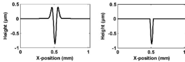
Fig. 3—(a) \nabla_{\text{asc},b} Second derivative of Gaussian function (DoG2) and (b) S_v valley feature (groove pattern).
