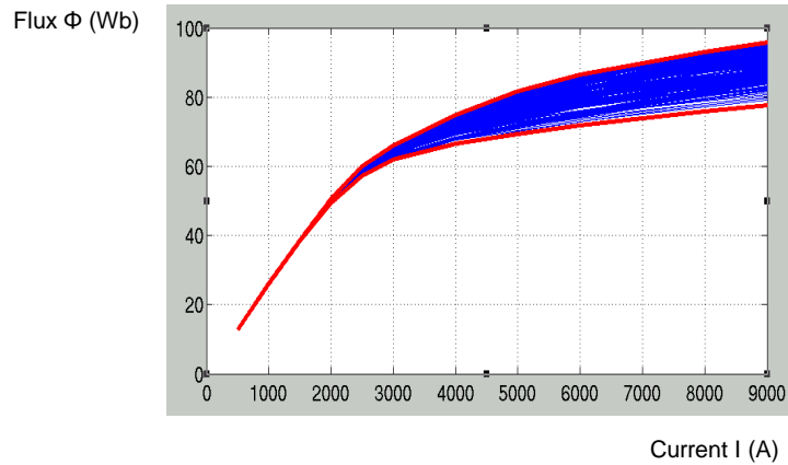
Fig. 6. 200 realizations of the flux \Phi versus the excitation current I
