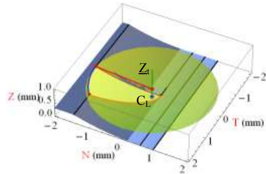
Fig. 7. Configuration C1: \beta_r = -1.5^\circ , \beta_n = 0^\circ
