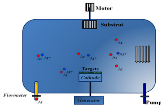
Fig.1. Experimental set-up used to deposited V or VN thin layers
