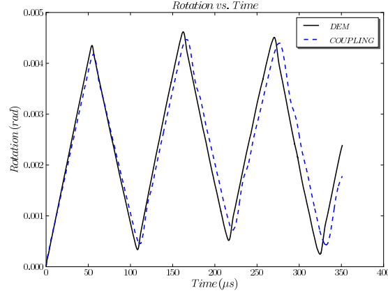
Figure 21: Test3: The free-end rotation \theta_x mean obtained by DEM, CNEM and the coupling method L_O = 10 mm, coarse Multiplier space , continuous differentiable weight functions, \varepsilon = 0.05
