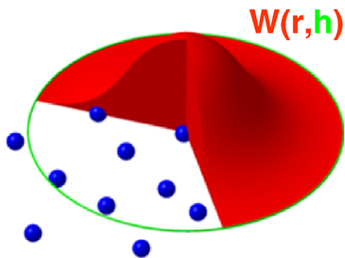
Fig. 7. Kernel approximation.
