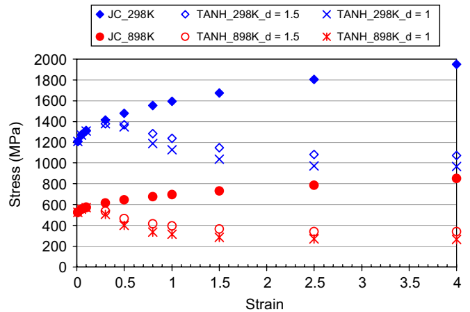
Fig. 2. Flow stress–strain curves versus temperature for Johnson–Cook (JC) law and the new TANH model for a strain rate of 10^4 \text{ s}^{-1} .
