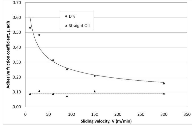
Fig. 9. Evolution of adhesive friction coefficient versus sliding velocity
