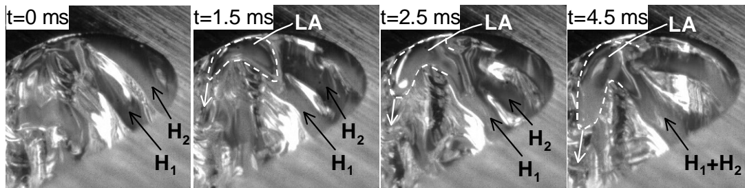
Figure 6. Example of melt accumulation dynamics observed for V = 1 m/min. A merger of two successive humps H_1 and H_2 is shown. The white dotted lines indicate approximate border of the liquid accumulation LA. As for the scale of the images, note that d_k = 1.74 mm.
