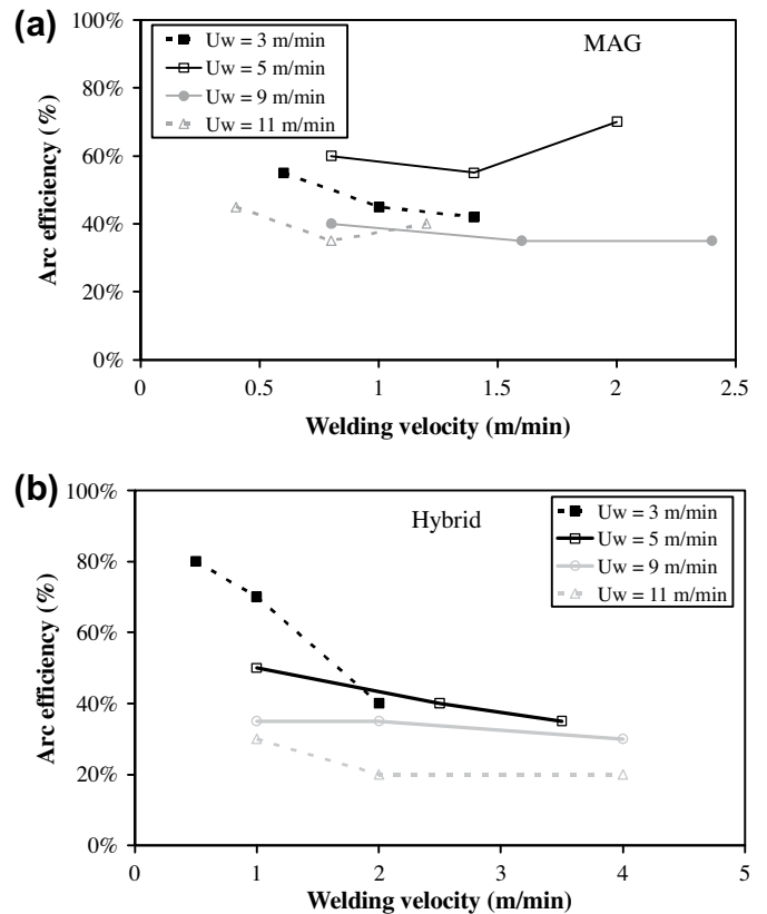
Fig. 7. Arc efficiency as a function of welding velocity at different wire feeding rates for MAG (a) and hybrid (b) processes.
