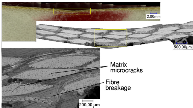
Fig. 17. Microscopic observations of section of KN sandwich (16 J impact).
