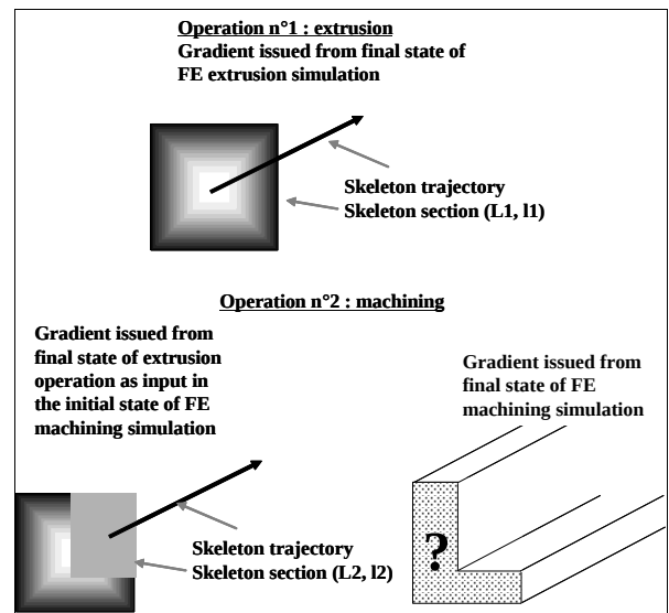
Figure 10: KBE data management supporting field transfer for manufacturing simulation.
