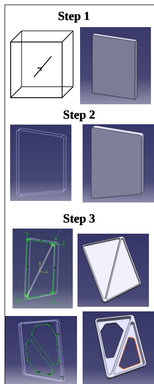
Figure 7: Illustration of the proposed DFM approach.
