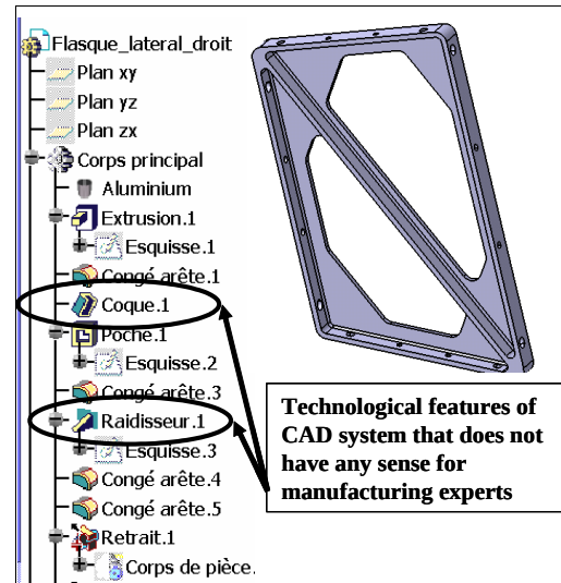
Figure 1: Incoherency between CAD model breakdown and manufacturing breakdown.
