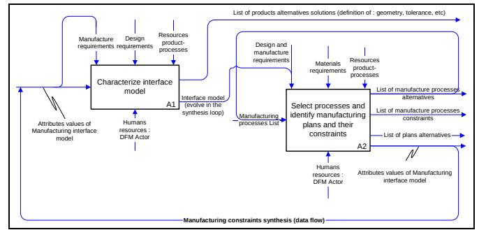
Figure 3: The DFM activity schematisation [RS1].
