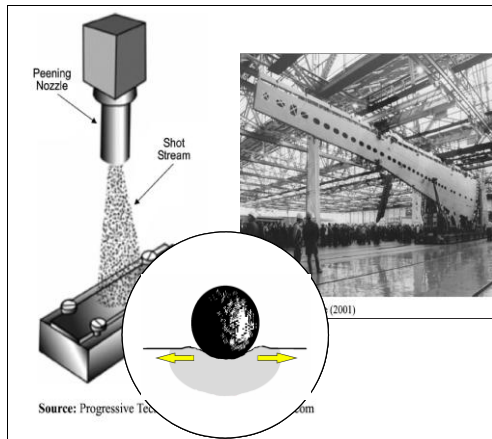
Figure 5: Illustration of the peen forming process.
