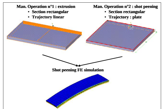
Figure 11: Illustration of manufacturing simulation with respect to manufacturing skeleton features.
