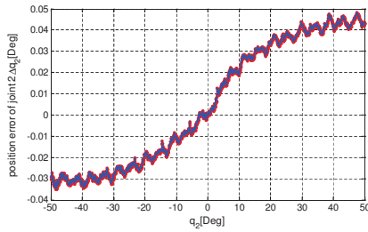
Fig. 9. Position error of joint 2
