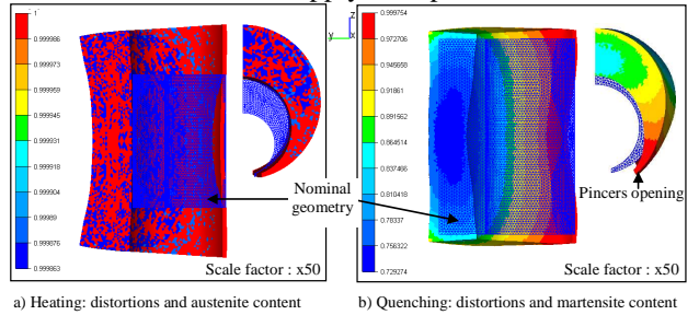
Figure 6: Distortions of a half simulated C-ring
