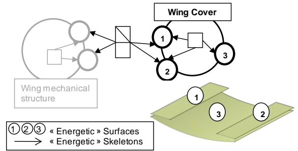
Figure 5: Energetic skin and skeleton of the Wing Cover and respective form features.
