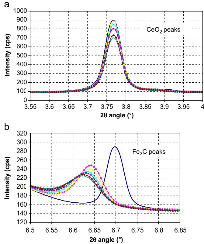
Fig. 6. Position of the diffraction peaks during loading: (a) \text{CeO}_2 peaks always at the same 2\theta angle, (b) Cementite peaks gradually shifted to smaller 2\theta angles ( \epsilon_{11} strain).
