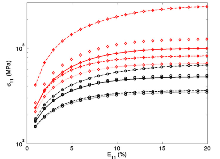
Fig. 11. Evolution of the model predictions when: the layer thickness \lambda is divided by a factor of 10 with respect to its value in Table 2, i.e. \lambda=0.03 \mu\text{m} (dashed lines), k_{gnd}=0 (dotted lines), an aspect ratio of 2 is accounted for in the tensile direction (mixed lines), an aspect ratio of 1.5 is considered normal to the tensile direction (full lines), and, particles are assumed spherical (no lines). The circles and diamonds denote the macroscopic stress and the stress in cementite particles, respectively.
