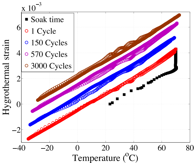
Fig. 4. Total in-plane hygrothermal strain ( \varepsilon_{ht}^L(T, N) ) versus temperature.
