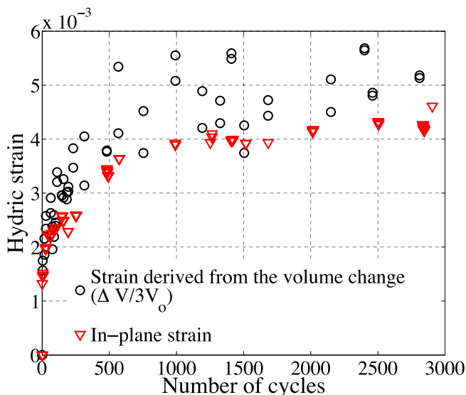
Fig. 6. Comparison between the in-plane hydric strain and the global strain derived from the volume change assuming isotropic hygroelastic behavior.
