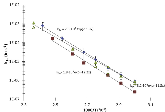
Figure A.1. Arrhenius graphs for the thermal initiation rate constant for: ♦ This work., ■ Richaud et al. [57], ▲ Achimsky [58], △ Achimsky et al. [56]. The value of pseudo-unimolecular kinetic rate constants are determined from the induction times using t_{\text{ind}} = 3/k_{1u} .
