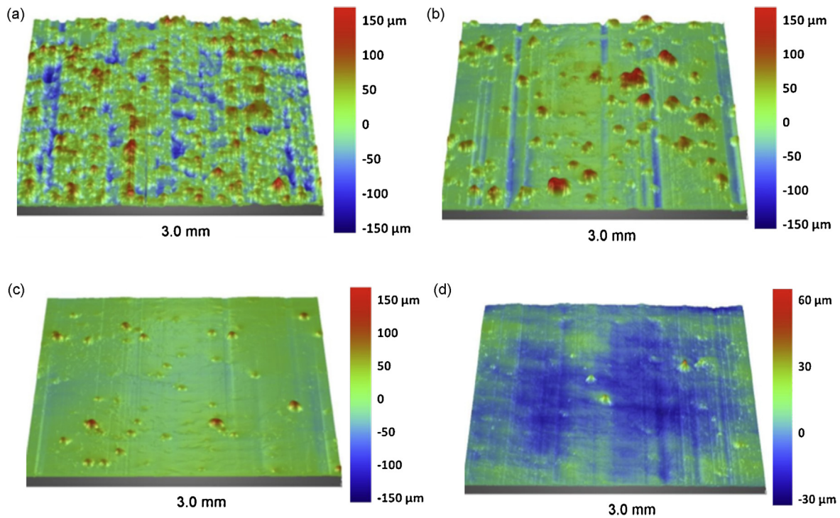
Fig. 10. 3D profiles of surface finish induced in pulsed regime ( P_{\text{peak}} = 500 \text{ W} - f = 60 \text{ Hz}, D_m = 1 \text{ g/min} ) (a) dc = 0.3 (non-filtered average roughness R_{a,nf} = 29 \mu\text{m} ), (b) dc = 0.5 ( R_{a,nf} = 17 \mu\text{m} ), (c) dc = 0.7 ( R_{a,nf} = 9 \mu\text{m} ), (d) dc = 0.9 ( R_{a,nf} = 5 \mu\text{m} ).
