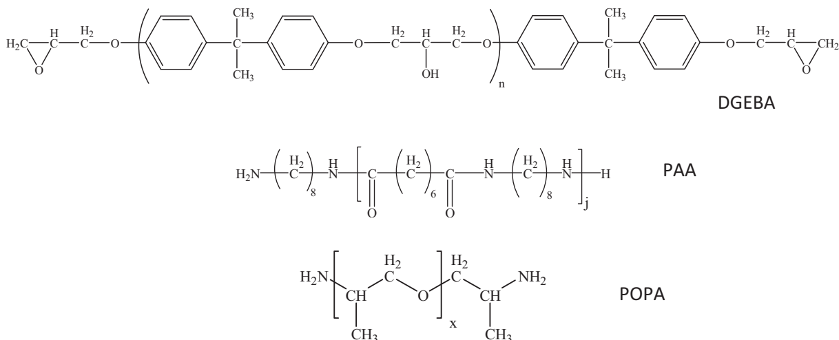
Fig. 2. Chemical structure of “monomers”.
