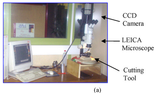
Fig. 4 – (a) The system of observation of wear and (b) a cutting edge measurement example.
