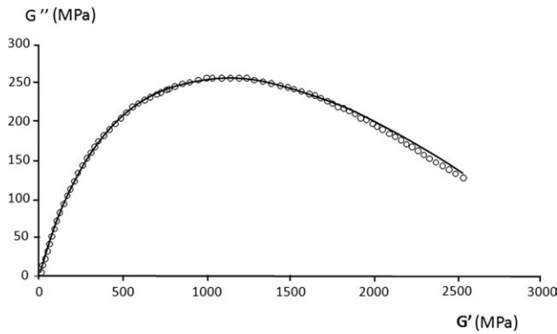
Figure 11. COLE-COLE diagram of virgin PU (before tensile test). Experimental data (○), Biparabolic model (solid curve).
