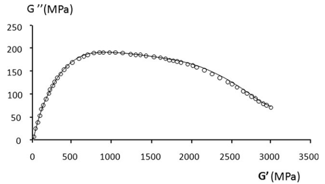
Figure 13. COLE-COLE diagram of PU sample after recovery test. Experimental data (○), biparabolic model (solid curve).
