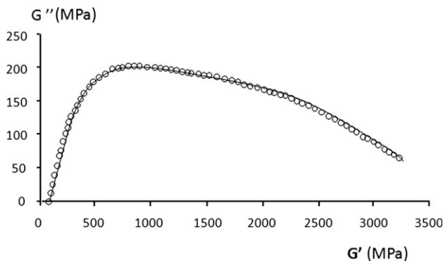
Figure 12. COLE-COLE diagram of PU sample after relaxation and before recovery test. Experimental data (○), biparabolic model (solid curve).
