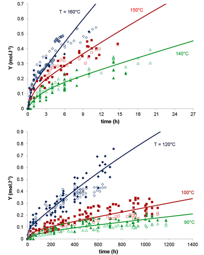
Fig. 9. Changes against time of exposure in the concentration of aldehyde chain-ends and broken C–N bonds in air between 90 and 160 °C. Comparison between theory (solid lines) and experiment (symbols). Concentrations of PH=O chain-ends and broken C–N bonds are represented by open and solid symbols respectively.
