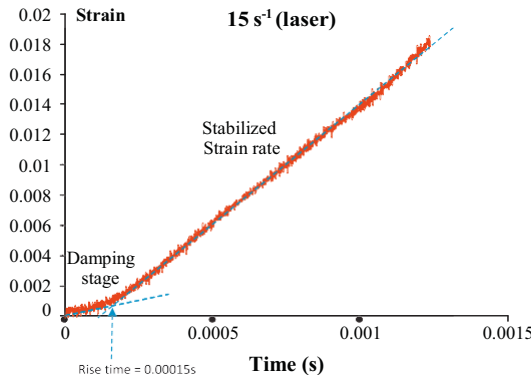
Fig. 6. (a) Measured strain versus time curve for a moderate speed tension test \approx 15 \text{ s}^{-1} . (b). Measured strain versus time curve for a high speed tension test \approx 208 \text{ s}^{-1} .
