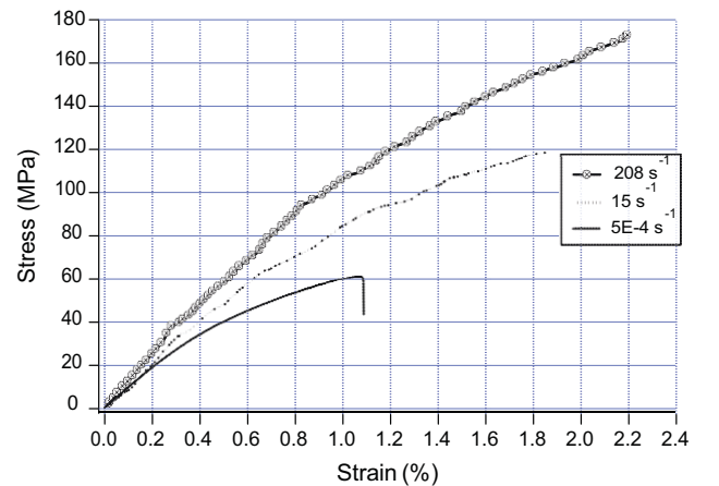
Fig. 7. Typical EPC matrix composite stress–strain tensile curves. The three characteristic stages can be shown for all strain rates.
