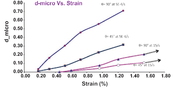
Fig. 14. Quasi-static and dynamic evolution of the microscopic damage indicator with respect to two specific in-plane orientations of fibers: h = 90^\circ and h = 45^\circ .
