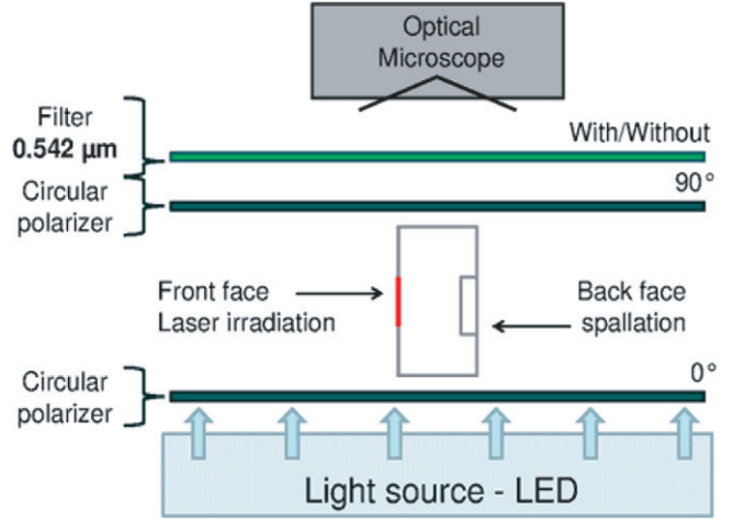
Figure 3. Photoelasticimetry experimental set-up to observe post-mortem state of epoxy samples [37–40].
