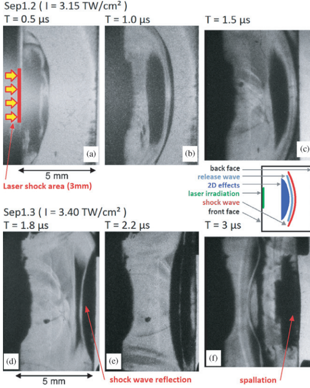
Figure 6. Laser shock wave propagation history obtained by shadowgraph: (a) snapshot at t = 0.5 \mu\text{s} : setting up of the shock wave (from sample Sep1.2), (b) snapshot at t = 1.0 \mu\text{s} : shock wave propagation with edge effect (from sample Sep1.2), (c) snapshot at t = 1.5 \mu\text{s} : the shock wave is reaching the target back face (from sample Sep1.2), (d) snapshot at t = 1.8 \mu\text{s} : reverberation of the shock at the free surface (from sample Sep1.3), (e) snapshot at t = 2.2 \mu\text{s} : crossing of release waves resulting in inside tensile stresses (from sample Sep1.3), (f) snapshot at t = 3.0 \mu\text{s} : beginning of the spallation mechanism (from sample Sep1.3).
