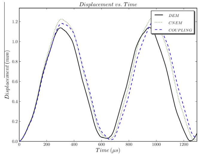
Fig. 20. Test2: The free-end displacements U_{y, mean} obtained by DEM, CNEM and the coupling method L_O = 10 mm, coarse multiplier space, continuous differentiable weighting, \varepsilon = 0.05 .
