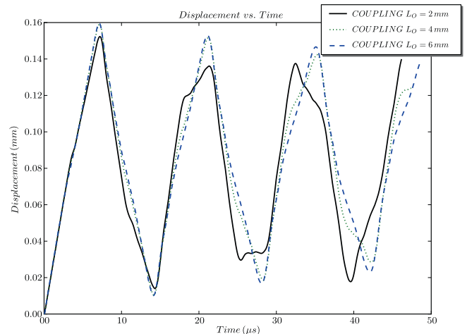
Fig. 17. The free-end displacements obtained using the coupling method for L_0 = 2 mm, L_0 = 4 mm and L_0 = 6 mm Coarse multiplier space, continuous weight functions, \varepsilon = 0.05 .
