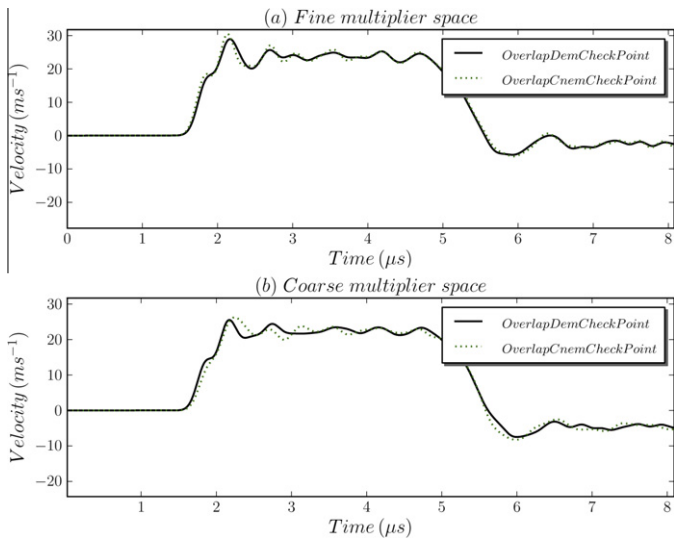
Fig. 15. Velocity comparison in the overlapping zone using fine and coarse multiplier spaces L_0 = 2 mm, continuous weight function, \varepsilon = 0.05 .
