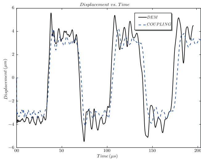
Fig. 22. Test4: The free-end displacement U_x mean obtained by DEM and the coupling method L_0 = 10 mm, coarse multiplier space, continuous differentiable weight functions, \varepsilon = 0.05 .
