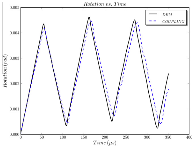
Fig. 21. Test3: The free-end rotation \theta_x mean obtained by DEM, CNEM and the coupling method L_0 = 10 mm, coarse multiplier space, continuous differentiable weight functions, \varepsilon = 0.05 .
