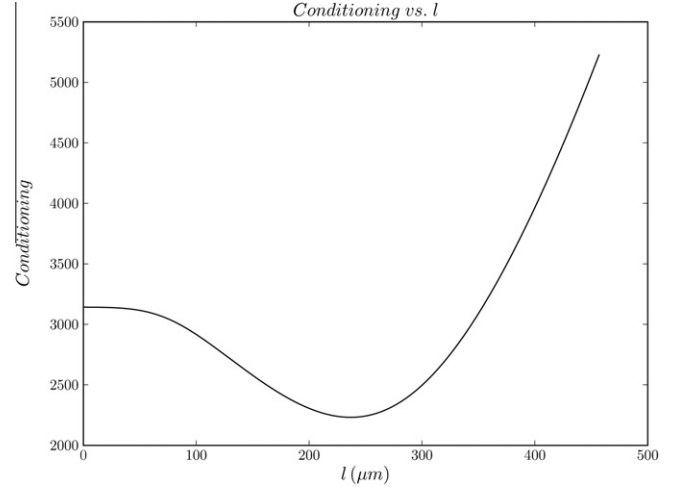
Fig. 7. Conditioning of A with respect to l . L_0 = 6 mm, coarse multiplier space, continuous weight functions with \varepsilon = 0.005 .
