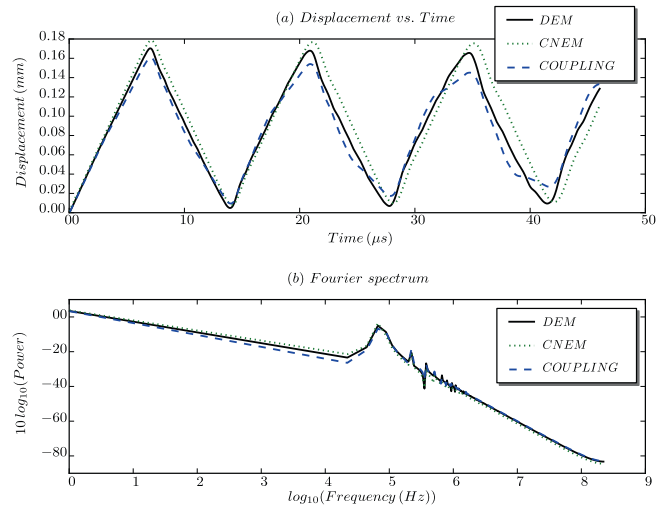
Fig. 13. The free-end displacements obtained using DEM and CNEM separately and the coupling method, and the associated spectral analyses (computed from FFT) L_0 = 2 mm, fine multiplier space, continuous weight functions, \varepsilon = 0.05
