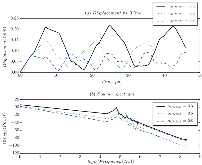
Fig. 10. The free-end displacements obtained using DEM and CNEM separately and the coupling method, and the associated spectral analyses (computed from FFT) for different weight constants. L_0 = 2 mm, fine multiplier space, constant weight functions \alpha_{CNEM} = 0.3 , \alpha_{CNEM} = 0.5 and \alpha_{CNEM} = 0.8 .
