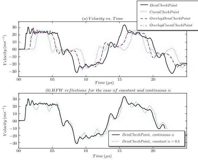
Fig. 14. The linear velocities (a) at the different check points for the case of continuous \alpha and (b) at the “DemCheckPoint” for the case of continuous and constant \alpha L_0 = 2 mm, fine multiplier space, continuous weight functions, \varepsilon = 0.05 .
