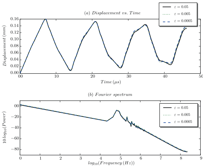
Fig. 12. The free-end displacements obtained using the coupling method, and the associated spectral analyses (computed from FFT) for different values of \varepsilon L_0 = 2 mm, fine multiplier space, continuous weight functions.
