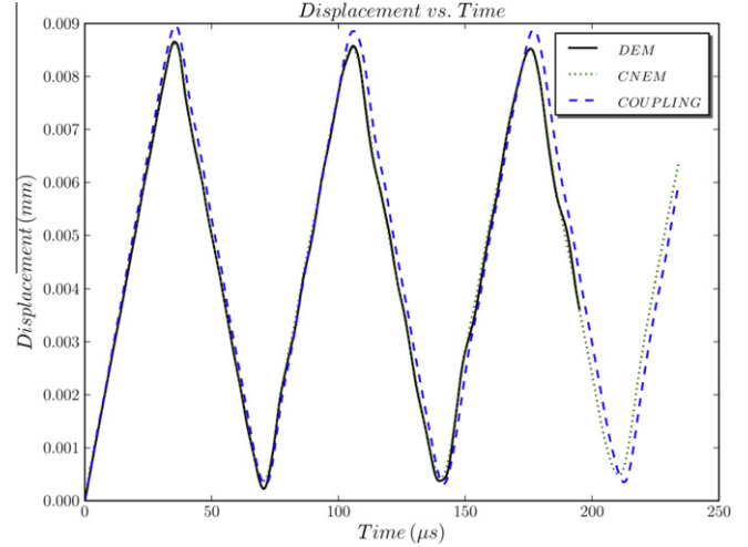
Fig. 19. Test1: The free-end displacements U_{x, mean} obtained by DEM, CNEM and the coupling method L_O = 10 mm, coarse multiplier space, continuous differentiable weighting, \varepsilon = 0.05 .
