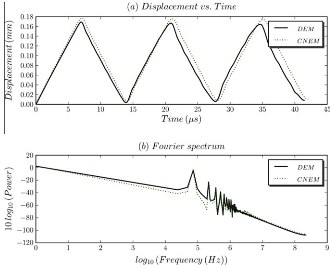
Fig. 6. The free-end displacements obtained using DEM and CNEM separately and the associated spectral analyses (computed from FFT).
