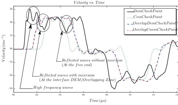
Fig. 9. The linear velocities at the check points for the first round trip. L_0 = 2 mm, fine multiplier space, constant weight functions \alpha_{CNEM} = 0.5 .
