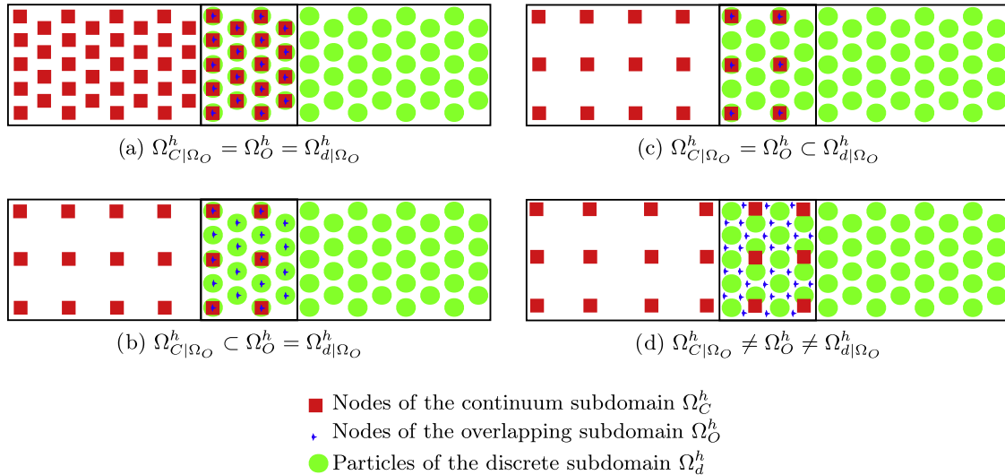
Fig. 3. The different configurations of the discretized subdomains.
