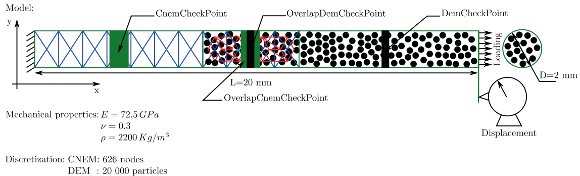
Fig. 4. Beam model of the parameter studies.
