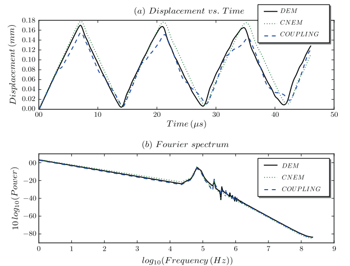
Fig. 8. The free-end displacements obtained using DEM and CNEM separately and the coupling method, and the associated spectral analyses (computed from FFT). L_0 = 2 mm, fine multiplier space, constant weight functions \alpha_{\text{CNEM}} = 0.5 .
