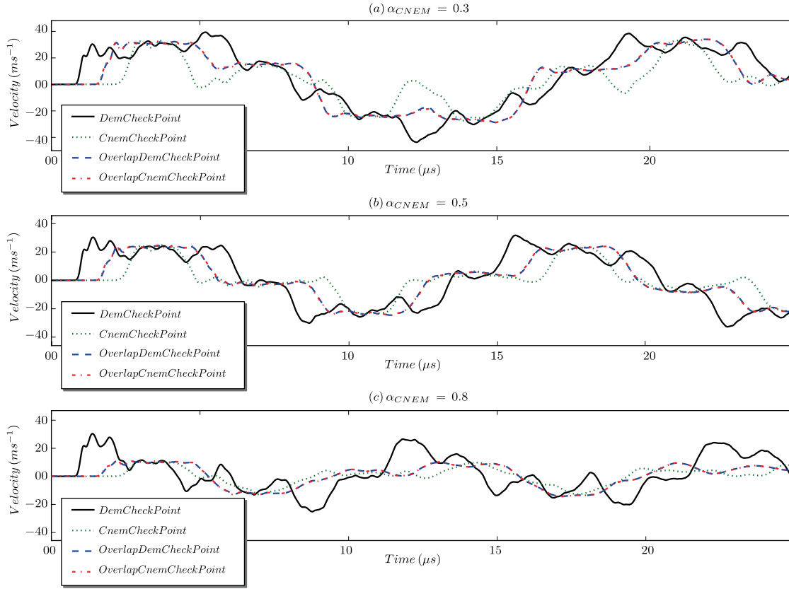
Fig. 11. The linear velocities at the check points for different weight constants L_0 = 2 mm, fine multiplier space, constant weighting \alpha_{CNE} = 0.3 , \alpha_{CNE} = 0.5 and \alpha_{CNE} = 0.8 .
