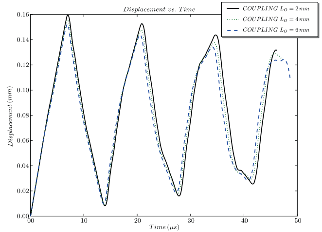
Fig. 16. The free-end displacements obtained using the coupling method for L_0 = 2 mm, L_0 = 4 mm and L_0 = 6 mm. Fine multiplier space, continuous weight functions, \varepsilon = 0.05 .
