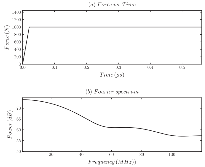
Fig. 5. Tensile loading of study model and the associated spectral analysis (computed from FFT).
