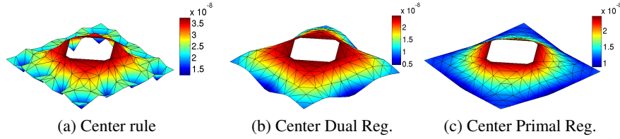
Figure 6. Gap observations obtained using the center integration rule for contact, observed on the rich 3x3 rule Gauss points Delaunay triangulation, \epsilon = 10^{-5}
