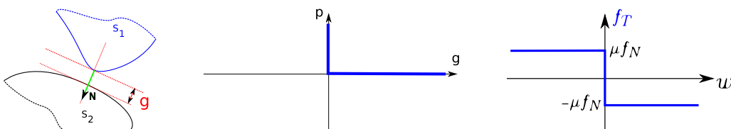
Figure 2: Contact normal ( N ) and gap ( g ) definition between solids, Signorini and Coulomb laws
