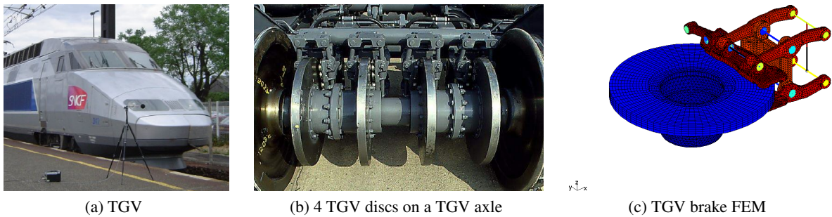
Figure 11: The TGV brake system
