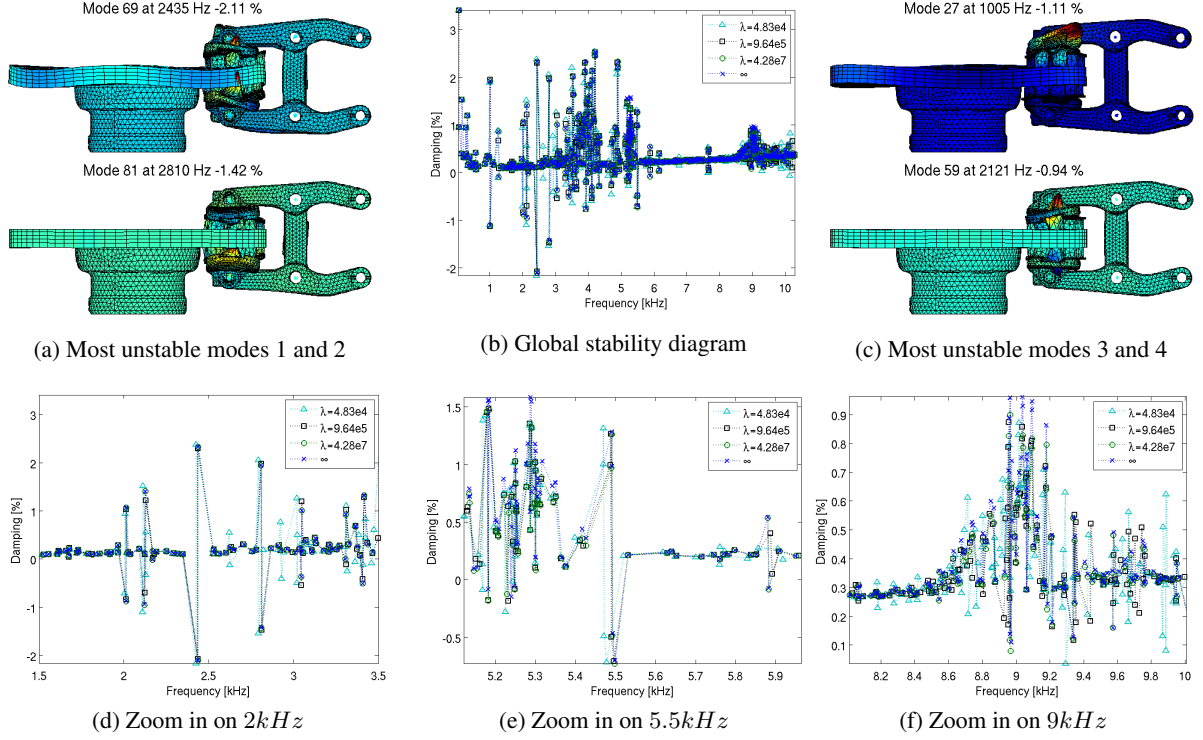
Figure 15: Stability diagrams of Signorini solutions and functional law solutions. Most unstable TGV modes
