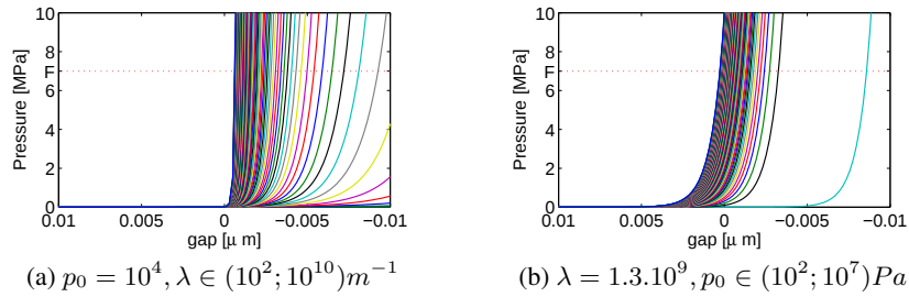
Figure 9: Exponential contact law evolution as function of its parameters
