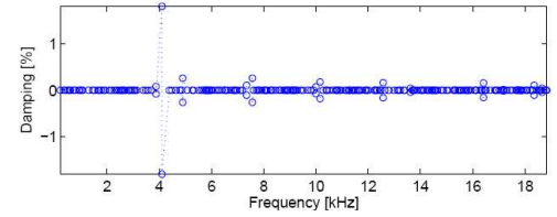
Figure 5. Brake stability diagram at 12 Bar
