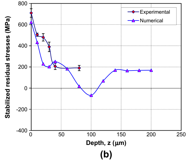
Fig. 16. Comparison between numerical and experimental profiles of stabilized residual stresses under 4-point bending test: (a) longitudinal stresses ( \sigma_{Rxx} ) and (b) transversal stresses ( \sigma_{Ryy} ).
