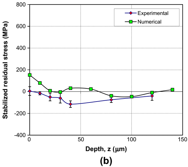
Fig. 15. Comparison between numerical and experimental profiles of stabilized residual stresses under 3-point bending test: (a) longitudinal stresses ( \sigma_{Rxx} ) and (b) transversal stresses ( \sigma_{Ryy} ).
