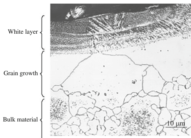
Fig. 5 White and heat-affected layers induced by EDM
