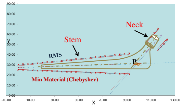
Fig. 3. 2D Demonstration of measurement through CMM
