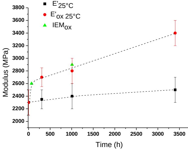
Figure 5: Global storage modulus E'\{298\text{K}\} versus exposure time at 200^\circ\text{C} in air. Comparison with average values of storage modulus E'\{ox, 298\text{K}\} and average indentation elastic modulus E^i\{ox, 298\text{K}\} of oxidized layer.
