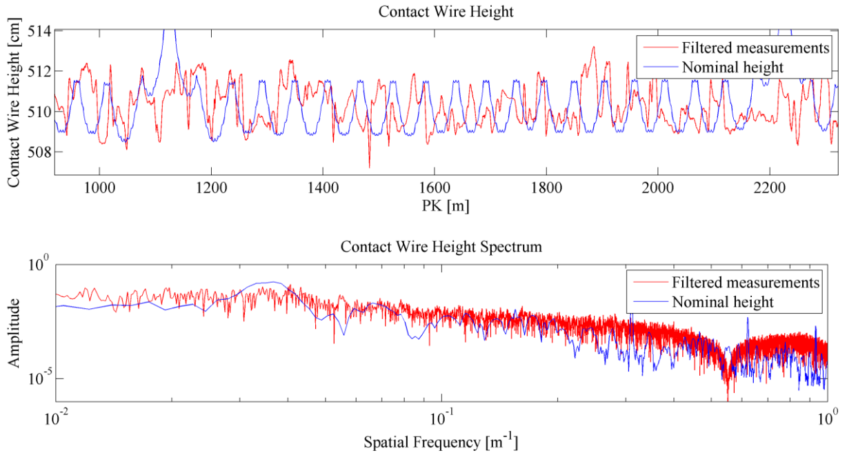
Figure 1 Filtered measurements (red) and nominal (blue) contact wire height (top) and contact wire height spatial-spectrum (bottom)
