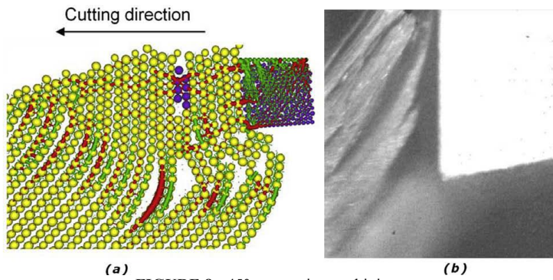
FIGURE 8. -45° composite machining.
