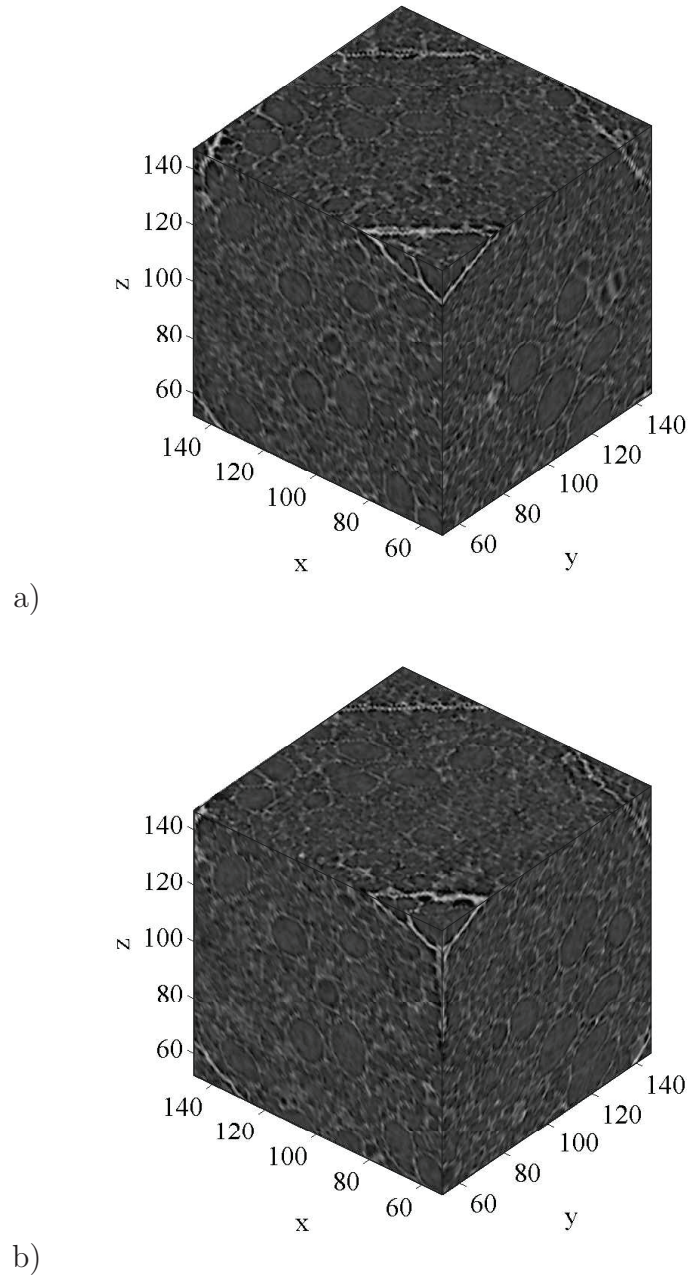
Fig. 1. View of the 96 voxel element volume analyzed in this study (a: reference, b: deformed configurations). A 14-bit deep grey level digitization is used.
