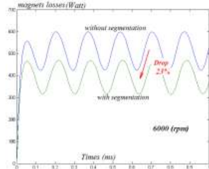
(c) Dynamic magnet losses calculated using 2D finite elements model
