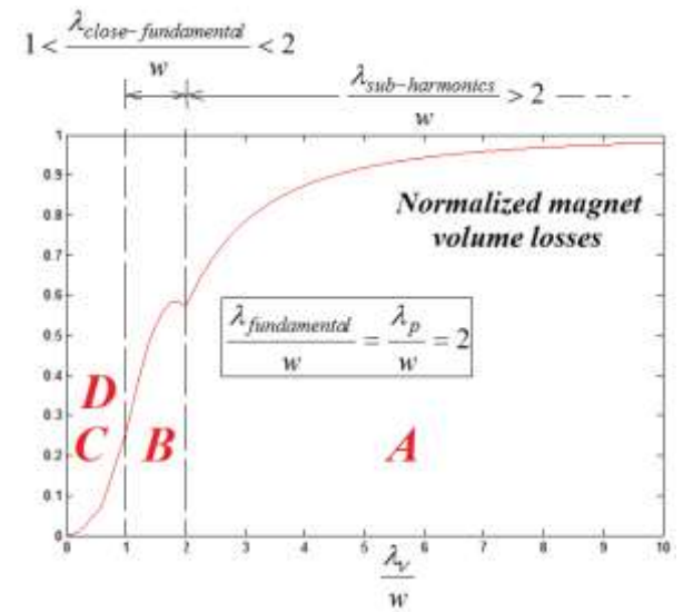
Fig. 6 Impact of the wavelength \lambda_v of the MMF harmonics on magnet volume losses in SPM structure (according to the analytical model) for a given w magnet width
