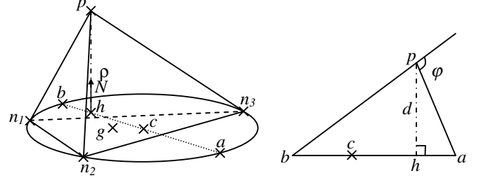
Fig. 9. Simplex angle and elevation of a vertex of the deformable mesh, used to regularise the mesh to obtain a smooth surface. p is the considered vertex, n_1, n_2 and n_3 are its neighbours, h is projection of p on the plane defined by the triangle n_1n_2n_3 , c is the centre of the circle circumscribing n_1n_2n_3 , a and b are the points of the circle aligned with (hc) , and g is the triangle's centre of gravity. Finally, d is called the elevation and \phi the simplex angle of p .
