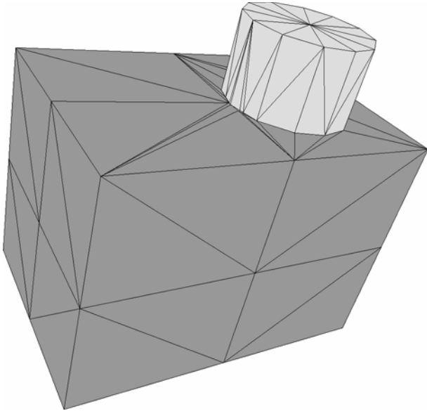
Fig. 18 Re-meshed assembly
