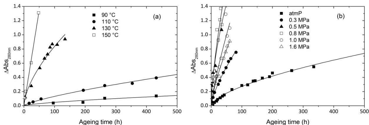
Fig. 9. Kinetic curves of 280 nm absorbance changes at various temperatures (a) and oxygen pressures at 110 °C (b)
