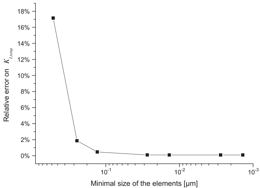
Fig. 8. Relative error on the stress intensity factor K_{I,temp} due to thermal stresses versus to the minimal element size for the finite element analysis.
